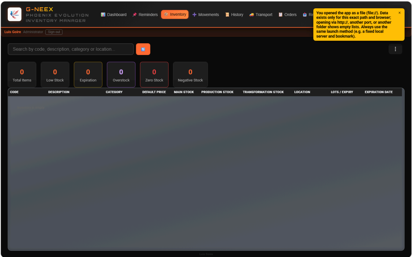
Inventory tab
